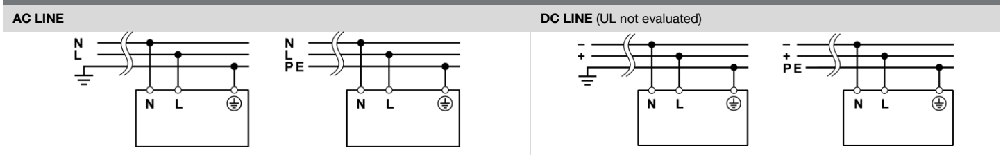
FIG.7 - INPUT CONNECTIONS
